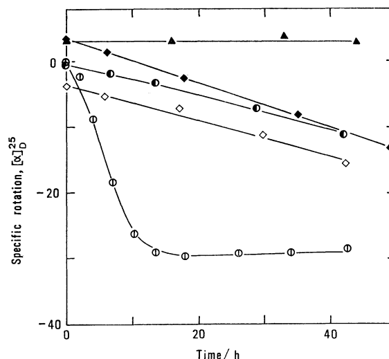
Fig. 2. Mutarotation of 2 .
